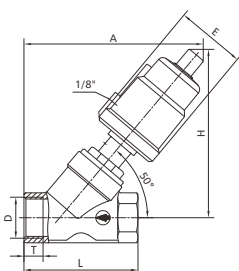
Female Connection Stainless Steel Actuator
